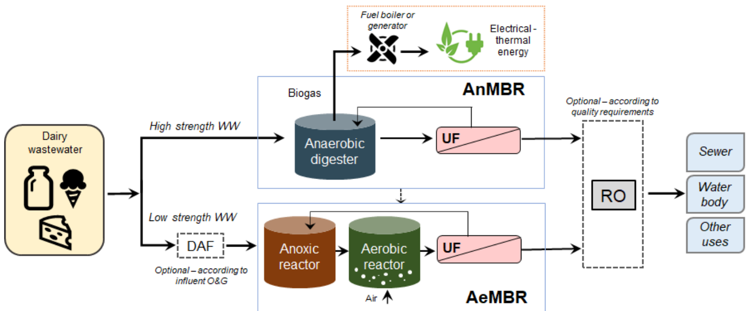
FIGURE 1. GENERAL APPROACH FOR DAIRY WASTEWATER TREATMENT WITH AEROBIC AND ANAEROBIC MBR TECHNOLOGY.
