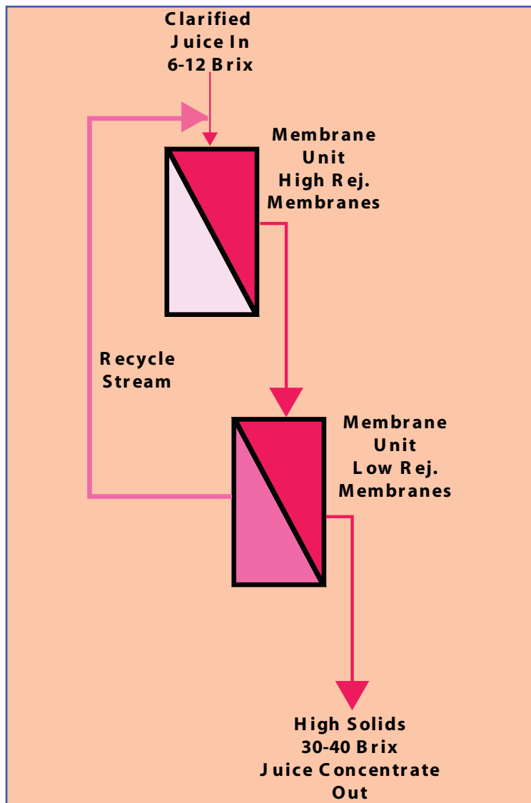
MEMBRANE CONCENTRATION OF JUICE
